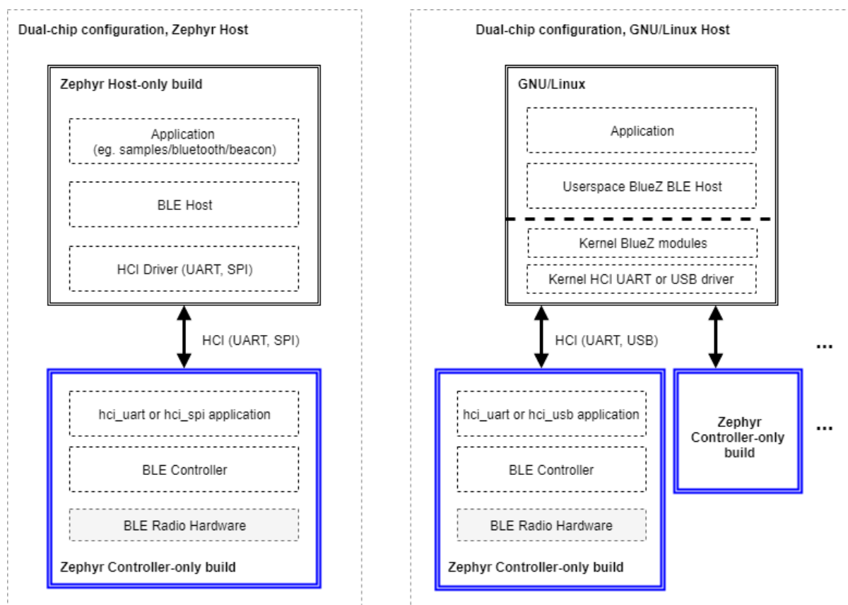
Fig. 2: Host-only and Controller-only builds on dual-chip configurations
